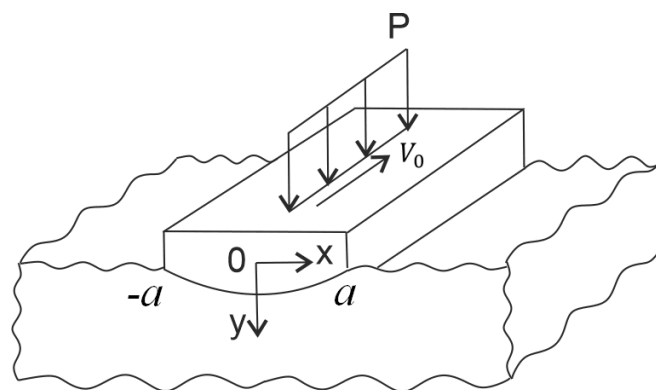
Fig. 3. Scheme of the tribological contact
